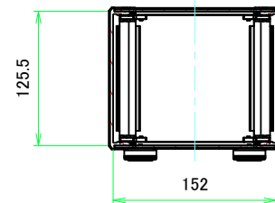
B-B (1:4.5)
